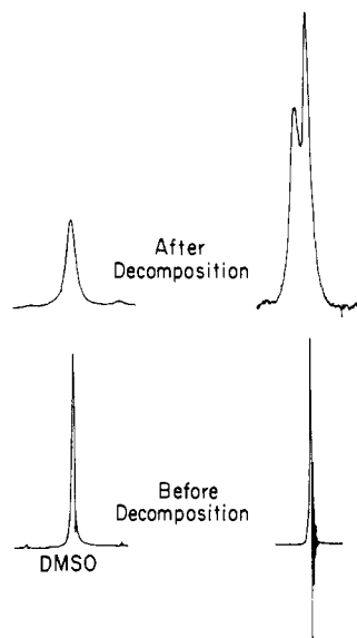
Figure 5. Proton NMR spectra of C_3H_{13}NO_3Si in Me_2SO before and after decomposition.
