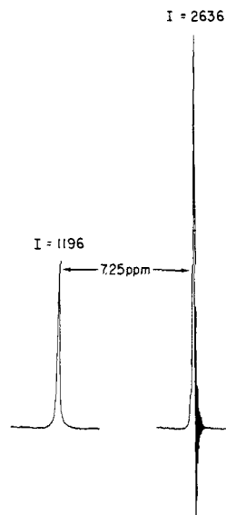
Figure 2. Proton NMR spectrum for the solid of empirical formula C_3H_{13}NO_3SSi in Me_2SO . Calculated integrals (I) are shown above each peak in arbitrary units.
